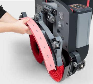
Two-click system: Tool-free replacement of the suction bar and rubber lips for quick changes.
